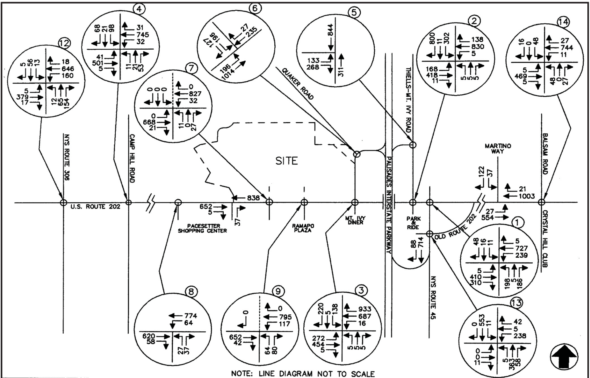
Figure 3.5-30: 2011 No-Build Traffic Volumes Weekday Peak AM Highway Hour (With Patrick Farm) Minisceongo Park Towns of Haverstraw & Ramapo, Rockland County, New York Source: John Collins Engineers, P.C. Date: October, 2008
